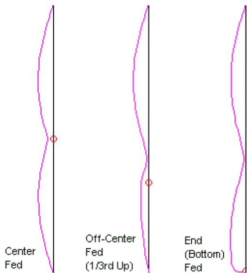
Current Magnitude Distribution on Reference Element at 24.94 MHz with Different Feedpoint Positions
