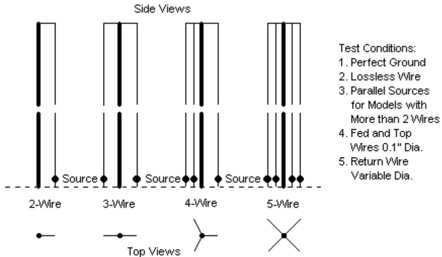
Configuration of Test Folded Monopole Models
