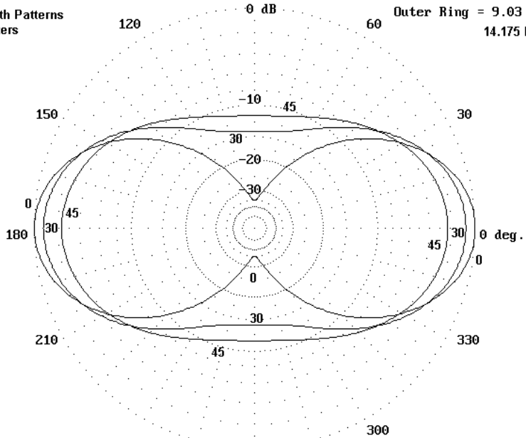
Elevation Patterns 20 Meters
