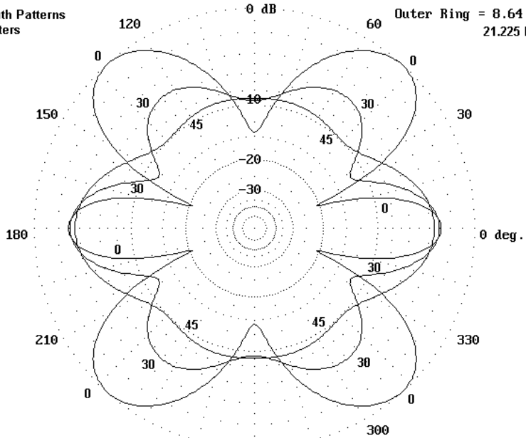
Elevation Patterns 15 Meters
