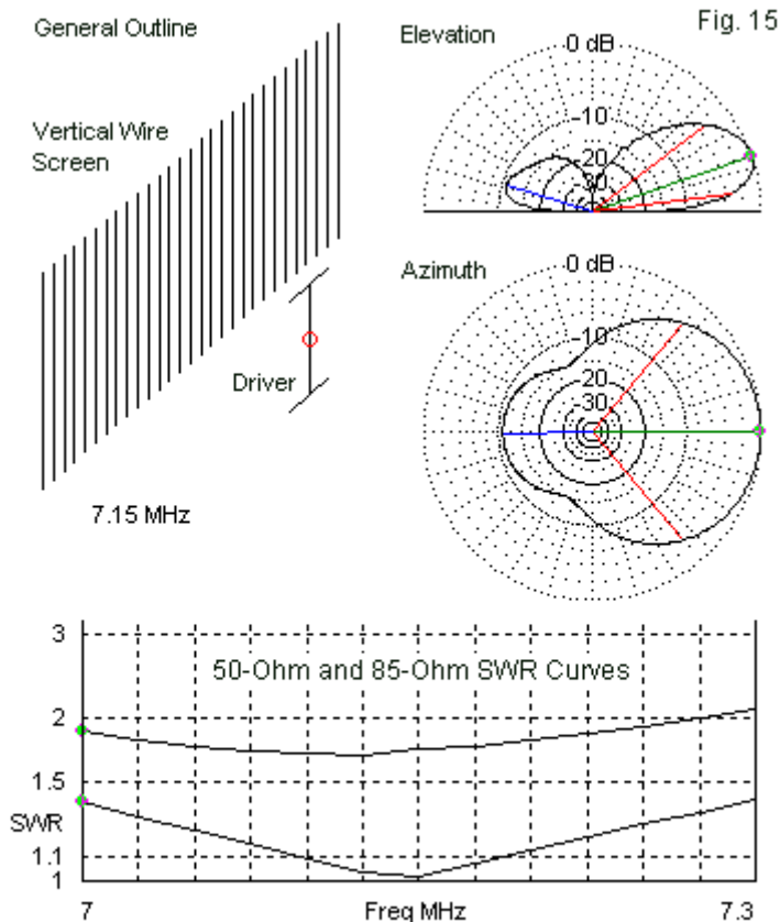
T-Cap Driver and Vertical Wire Screen Reflector with Patterns and SWR Curves
