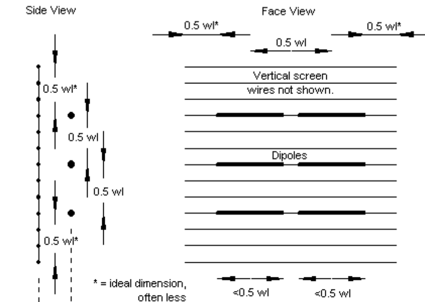
Generalized Dimensions for a Typical 3V-2H Dipole Array
