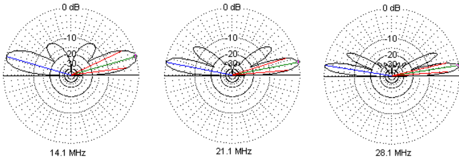
Selected Elevation Patterns for the "Lazy-8JK" Array
