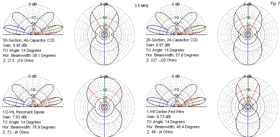
Horizontal CCDs and Comparators 1-Wavelength Above Average Ground
