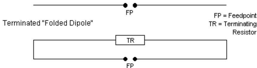
Basic Outlines: Equal Length Single-Wire Doublet and Wide-Band Terminated "Folded Dipole"
