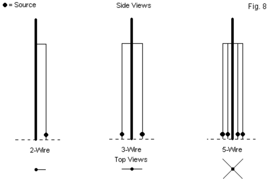
Some Alternatives to the Simple "Shunt" Feed
