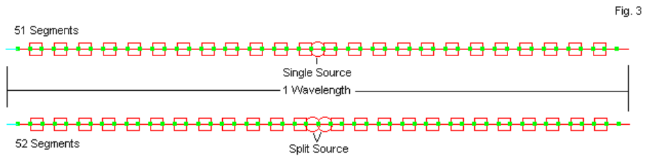
Two NEC Models of the 26-Section CCD
