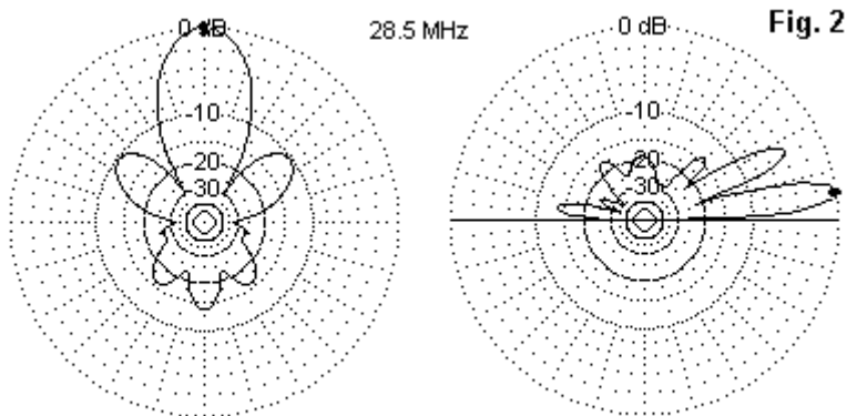
Curtailed Extended Lazy-H: 10-Meter Patterns
